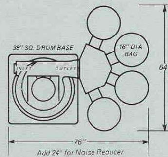
FLOOR PLAN Top View
