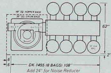
FLOOR PLAN Top View
